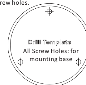
Figure 2-1 Drill Template
